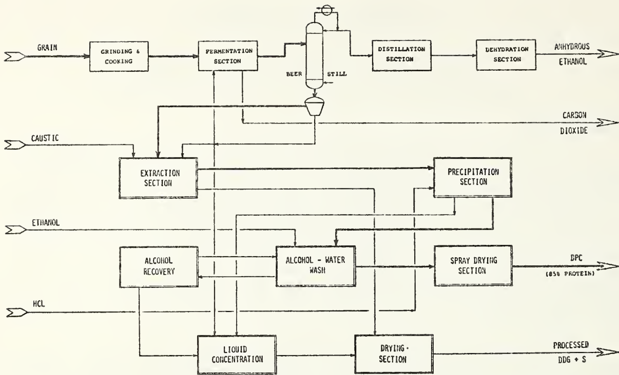
FIGURE 1 - Protein Recovery Process (Caustic Case).
